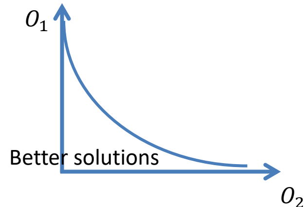
Minimization problem
