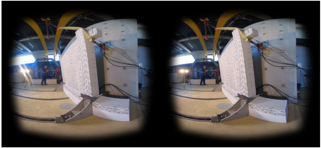
© Technical Mechanics, University of Osijek; Out-Of-Plane seismic tests on masonry walls
