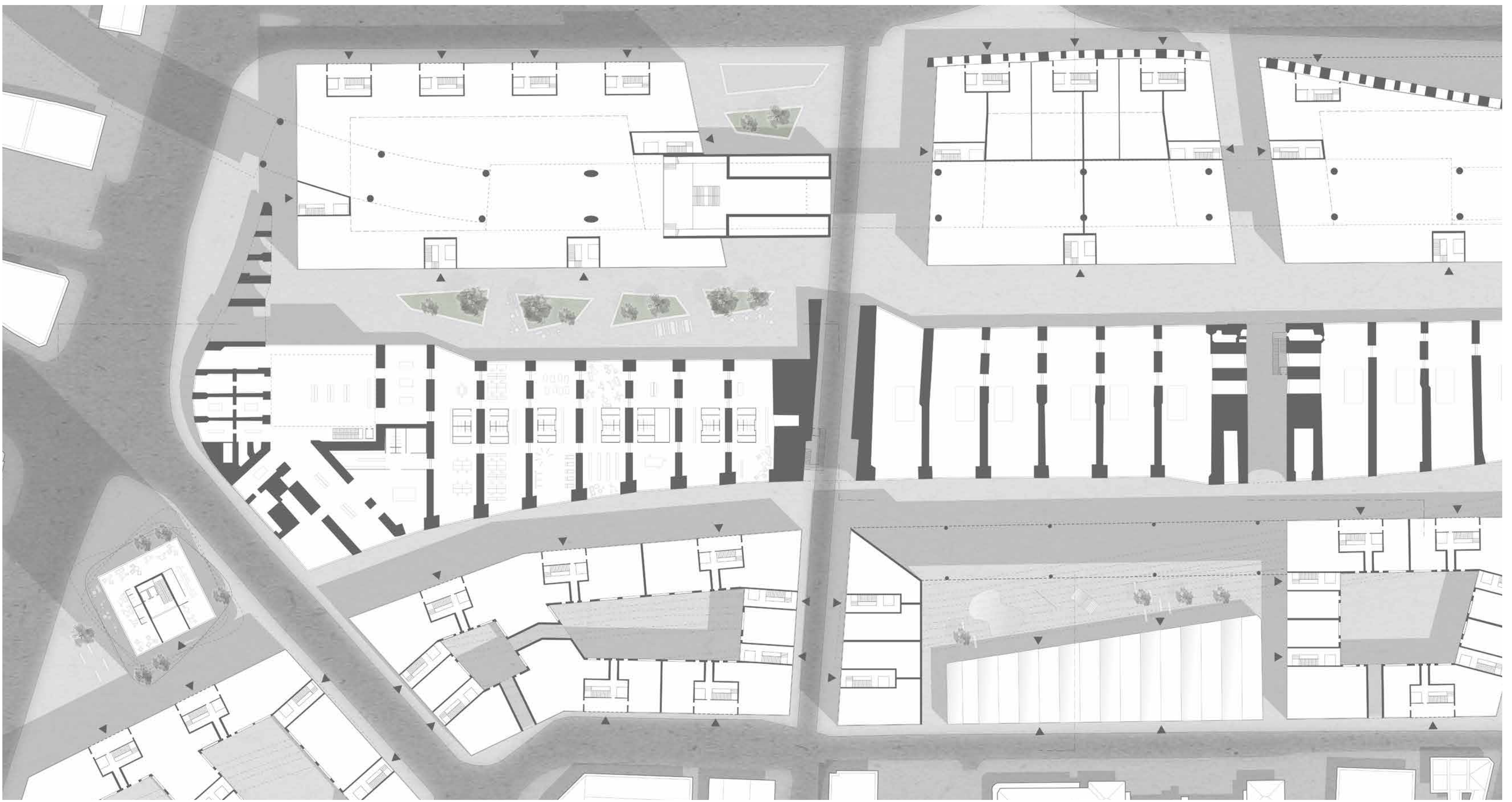
FLOOR PLAN 1/500
