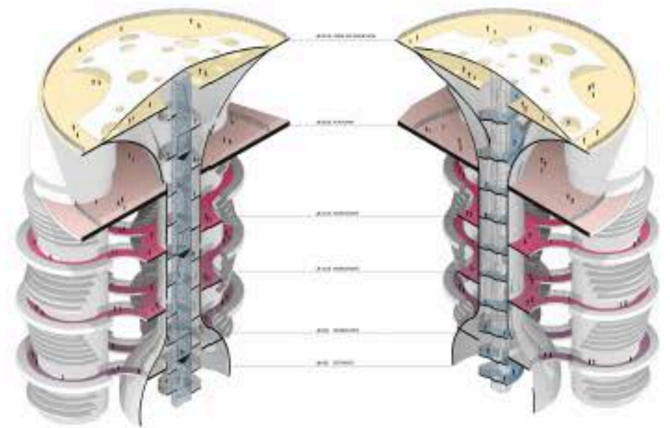
3D SECTION inside workshop tower
