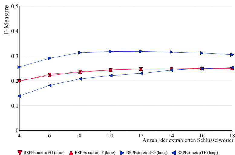
Abbildung 29: F-Measure RSPExtractor
