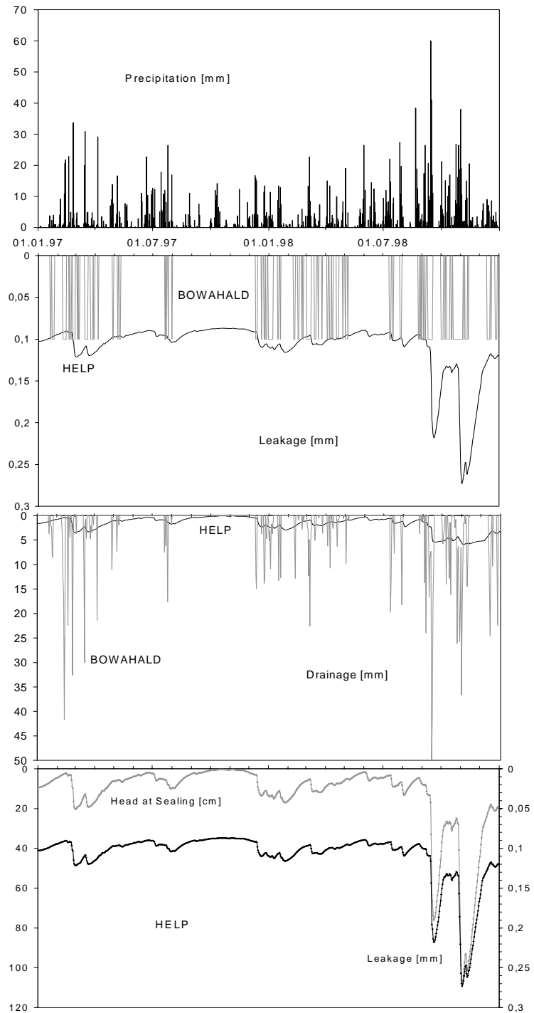
Figure 4. Precipitation [mm], leakage [mm], drainage [mm] and the combination of head [cm] and leakage [m] of HELP and BOWAHALD, NAD, Sonneberg, 1997 / 1998.
