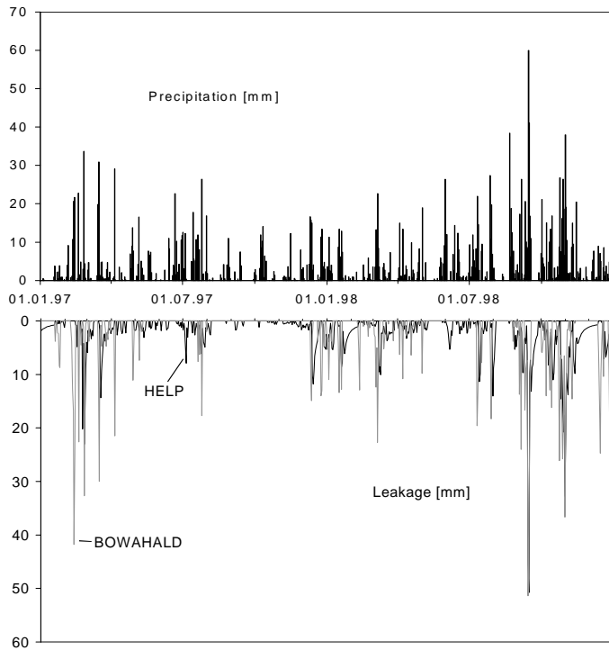
Figure 3. Precipitation [mm] and leakage [mm] of HELP and BOWAHALD, NA, Sonneberg, 1997 / 1998.
