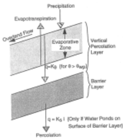
Figure 1. Schematic representation of water balance computing by HELP (Khire et al., 1997)
