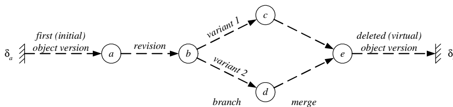
Figure 4: Version history and kinds of object versions
